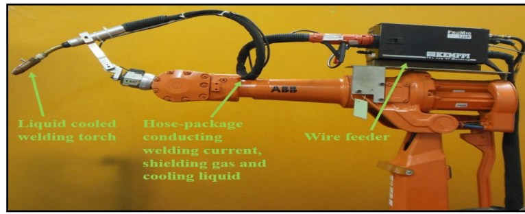
Figure 4. Robotic Arm Welding ABB IRB 2400/16 with GMAW Kemppi Pro-Evolution ProMIG 540 MX
